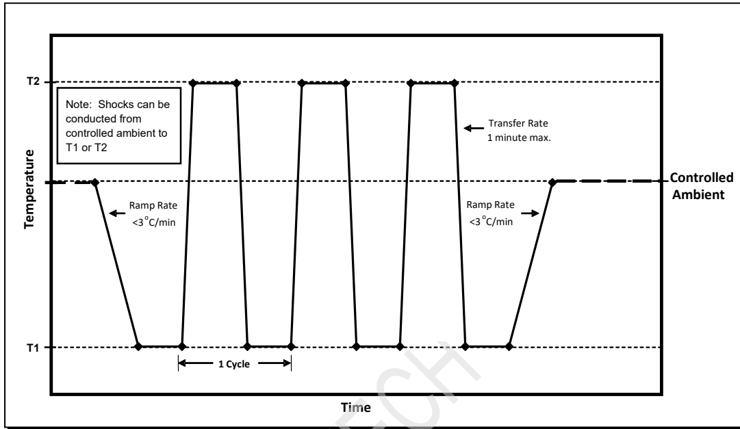
Figure 503.7-3. Multi-cycle Shocks.
